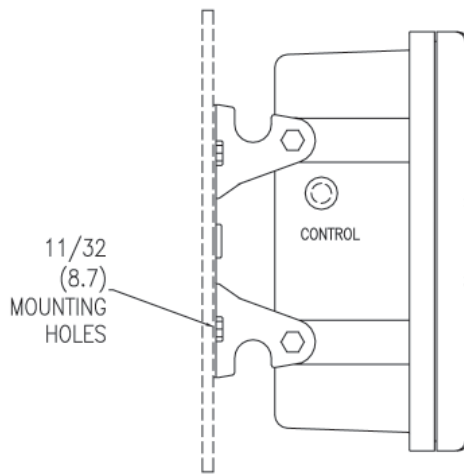
Wall Mounting
