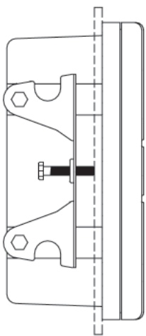
Panel Mounting
